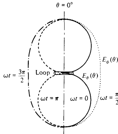
Fig. 2.10 Normalized E-Field Patterns of a Traveling Wave Loop Antenna; Linear Scale
