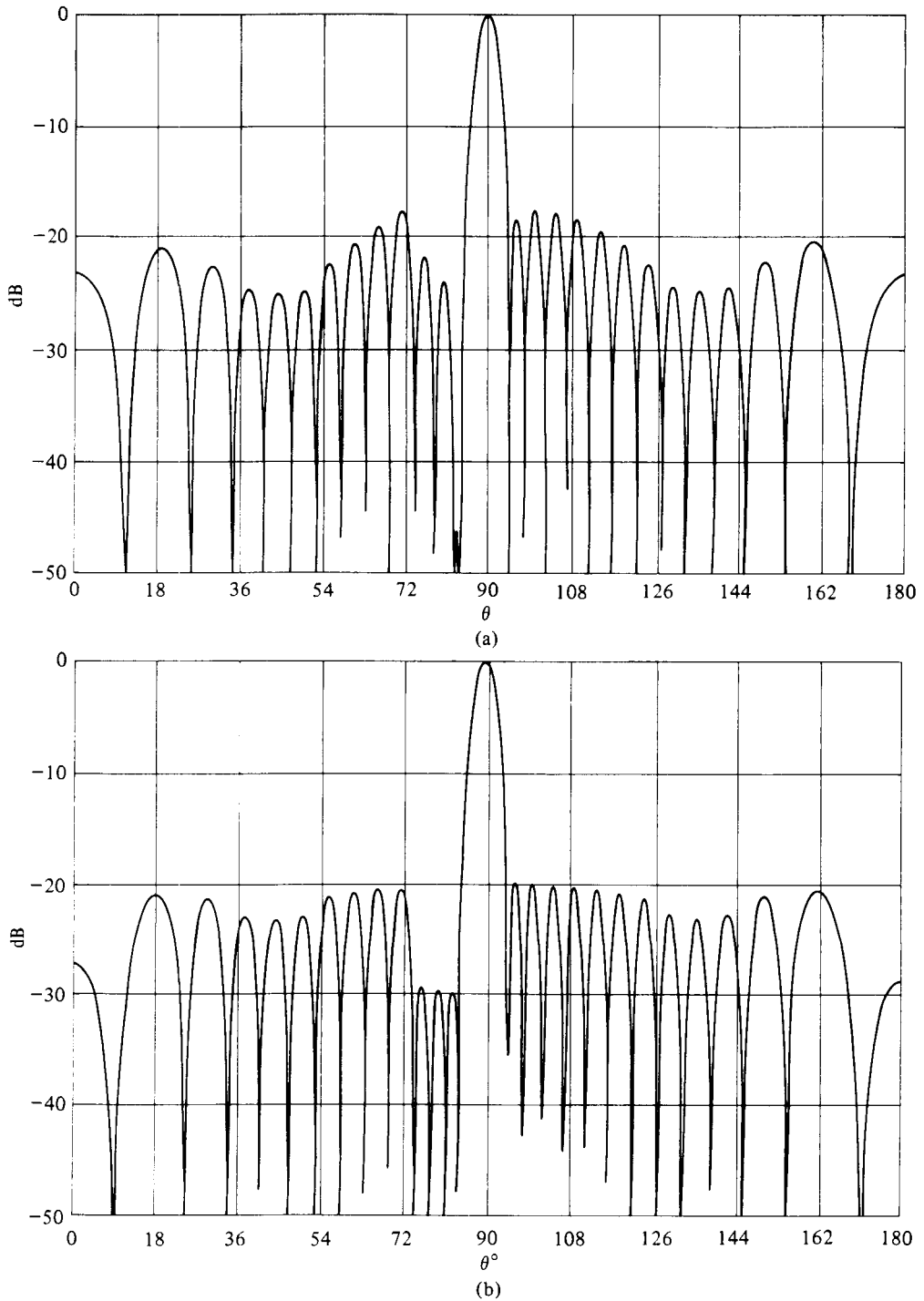
Fig. 5.17 The Sum Pattern of a 19-Element Linear Array, d = 0.7\lambda ; Design Goal: Achieve Pattern of Fig. 5.13; Excitation: in (a), Conventional Sampling; in (b), Root Matching (© 1977 IEEE. Reprinted from IEEE AP Transactions , pp. 617–621, 1977.)
