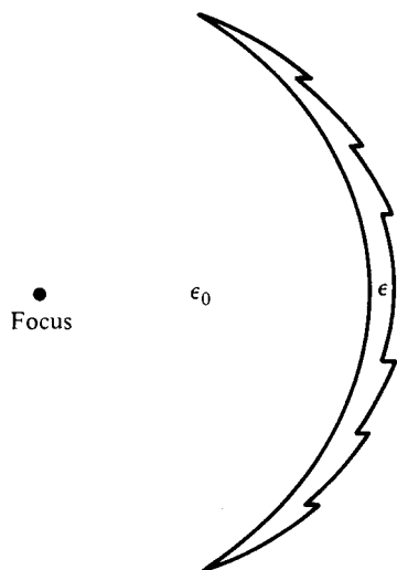
(c) Elliptical lens—stepped ellipse
