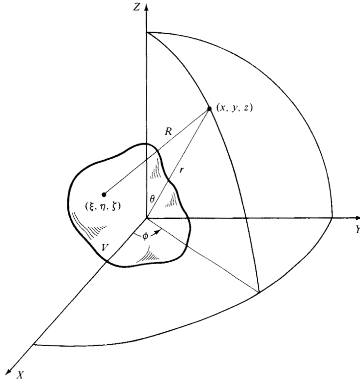
FIG. 1.2 Notation for Far-Field Analysis.
