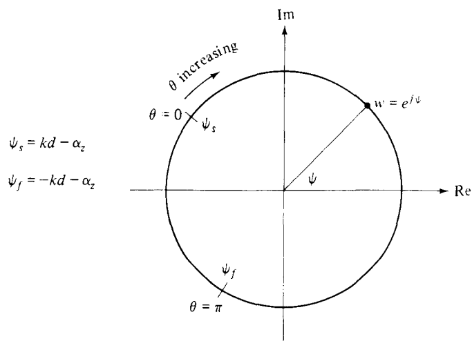
Fig. 4.11 Schelkunoff's Unit Circle
