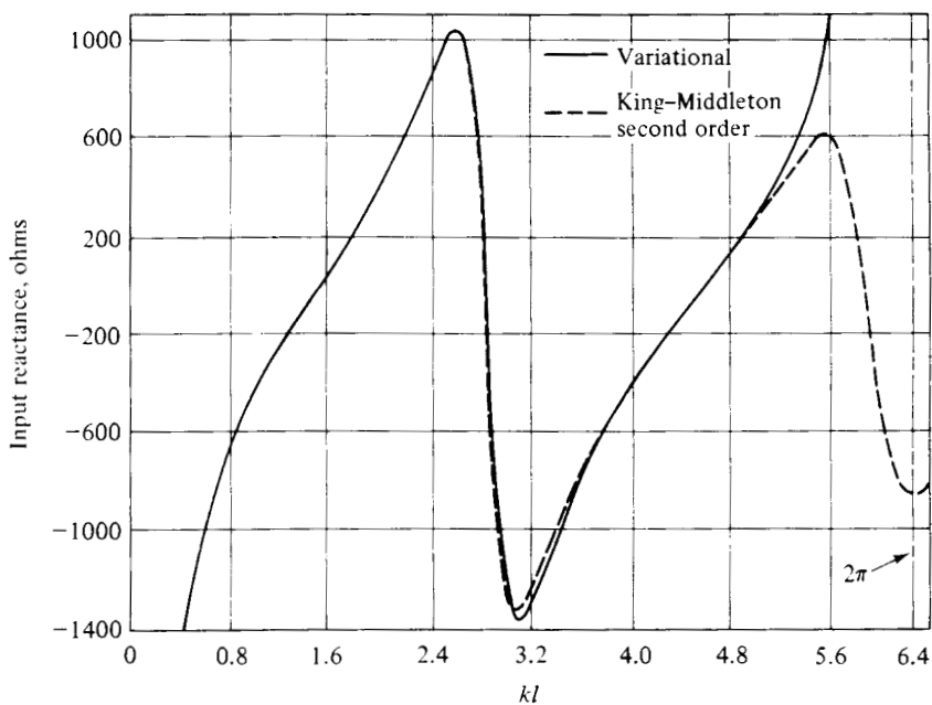
Fig. 7.16 A Comparison of Storer's Variational Solution and King-Middleton Second Order Values for the Input Impedance of a Center-Fed Cylindrical Dipole; \Omega = 2\ln(2/a) = 15 (Reprinted from J. E. Storer, Cruft Laboratory Report No. 101, 1950, Courtesy of Harvard University.)
