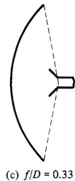
Fig. 10.10 The Effect on Reflector Depth and Feed Size of the f/D Ratio
