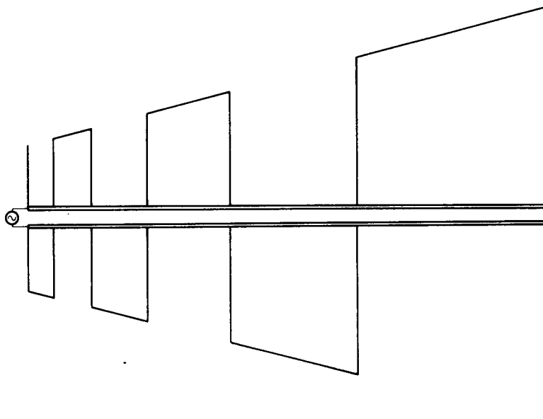
Fig. 8.25 An Improperly Fed Log-Periodic Dipole Array
