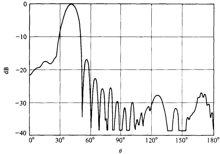
Fig. 9.25 Principal Plane Pattern (Experimental) for a Serrated Waveguide Antenna; L = 7.75\lambda , \nu = 9 GHz; Aperture Distribution = 1 + \sin(\pi\zeta/L) (© 1957 IEEE. Reprinted from K. C. Kelly and R. S. Elliott, IRE AP Transactions , 1957.)
