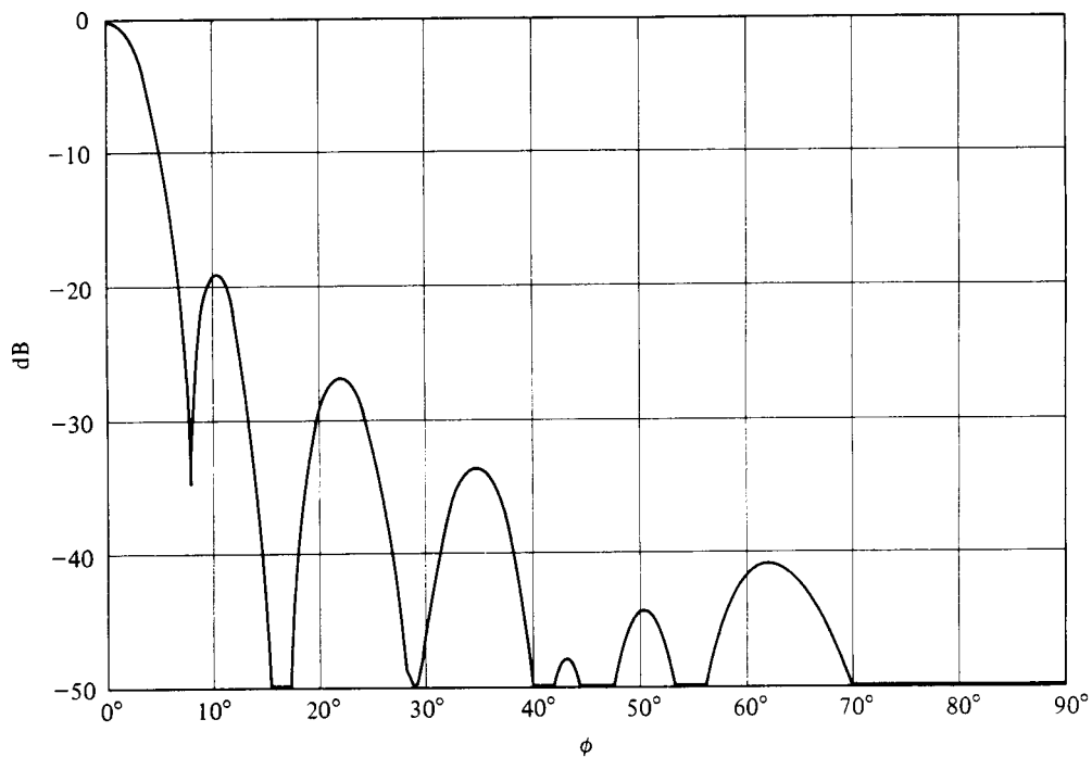
Fig. 10.25 Principal Plane Pattern of a Paraboloidal Reflector Antenna; Aperture Blockage Included; D = 10\lambda , f/D = 0.433 , 10 dB Spillover
