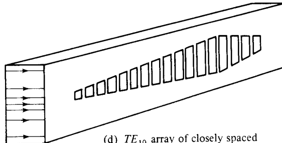
(d) TE_{10} array of closely spaced nonresonant slots in broad wall of rectangular waveguide. (serrated waveguide).
