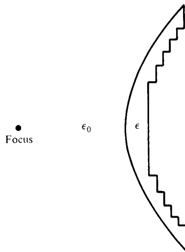
(b) Hyperbolic lens—stepped straight line
