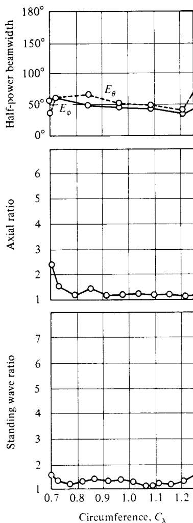
Fig. 8.8 Performance Data for a Six-Turn Helix with 14° Pitch (From Antennas by J. D. Kraus. Copyright 1950 McGraw-Hill. Used with permission of McGraw-Hill Book Company.)
