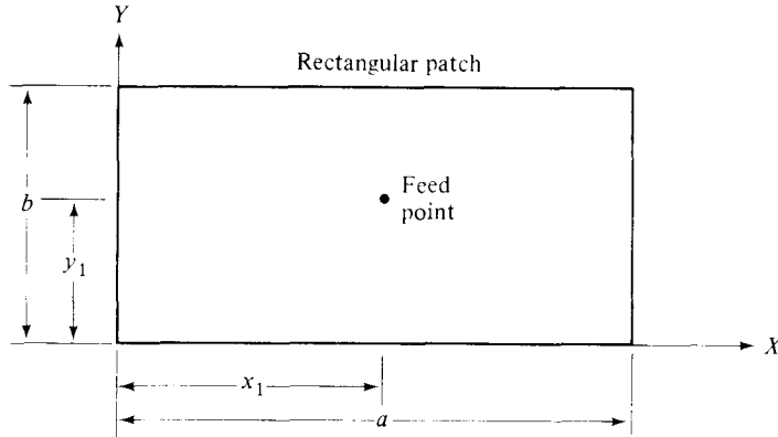
Fig. 7.30 A Rectangular Patch Antenna with a Coaxial Feed
