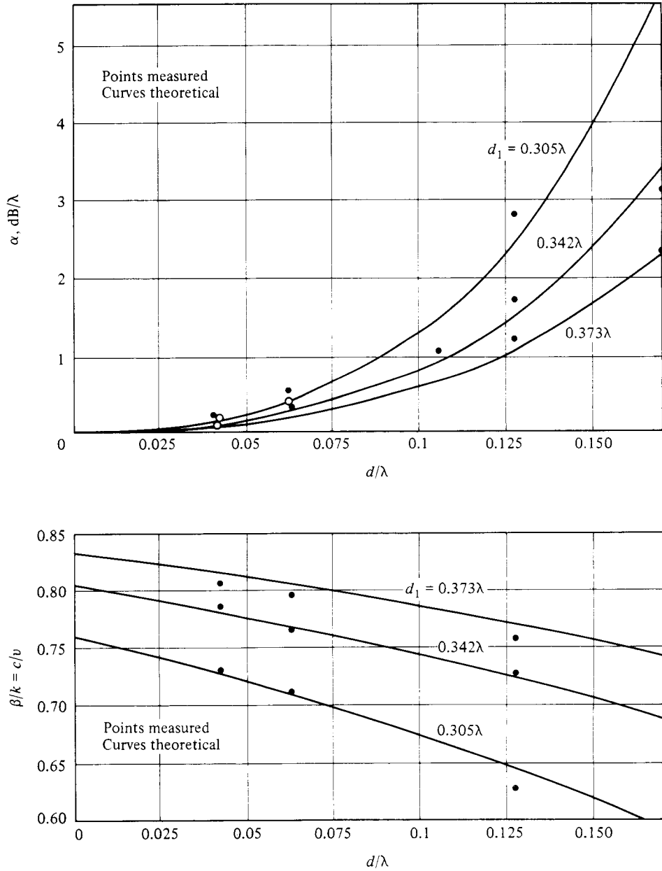
Fig. 9.28 Complex Propagation Constant for the Asymmetrical Trough Waveguide of Figure 9.27. (© 1959 IEEE. Reprinted from W. Rotman and A. A. Oliner, IRE AP Transactions , 1959.)
