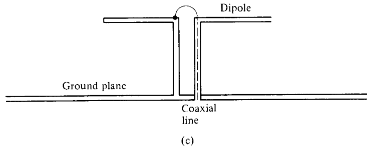
Fig. 8.3 A Center-Fed Dipole Above and Parallel to a Large Ground Plane; Various Feeding Arrangements
