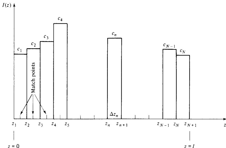
Fig. 7.5 The Use of Pulse Functions to Approximate the Current Distribution I(z) on a Center-Fed Dipole
