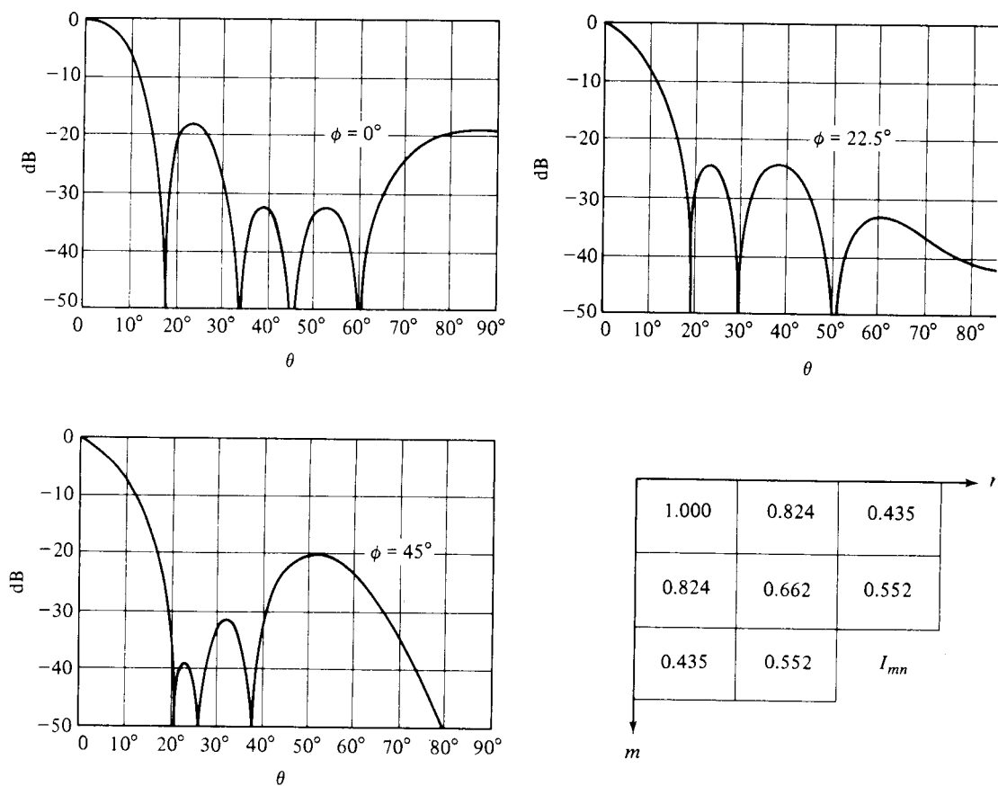
Fig. 6.18 Three \phi -Cuts of the Sum Pattern of the Array Shown in Fig. 6.17; d_x = d_y = 0.7\lambda ; Excitation Found by Conventional Sampling of a Continuous Circular Taylor Distribution, \bar{n} = 6 , -22 dB SLL
