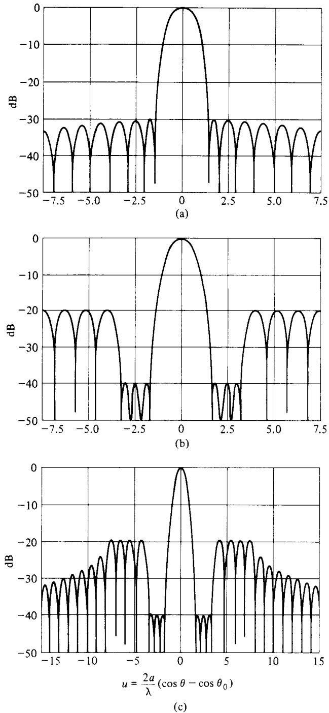
Fig. 5.11 The Evolution of a Symmetric Sum Pattern with Reduced Inner Side Lobes (© 1976 IEEE. Reprinted from IEEE AP Transactions , pp. 76–83, 1976.)
