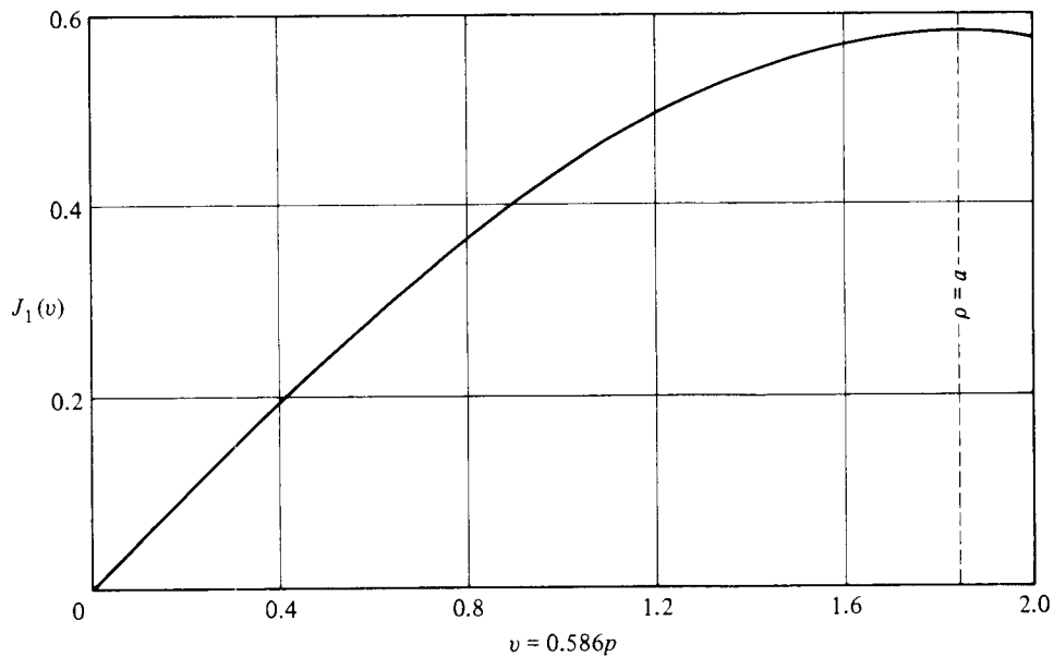
Fig. 6.31 The Aperture Distribution for the Generic Circular Difference Pattern
