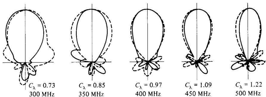
Fig. 8.7 Measured E-Field Patterns of a Six-Turn Helix with 14° Pitch; Polar Plots; Linear Scale (From Antennas by J. D. Kraus. Copyright 1950 McGraw-Hill. Used with permission of McGraw-Hill Book Company.)
