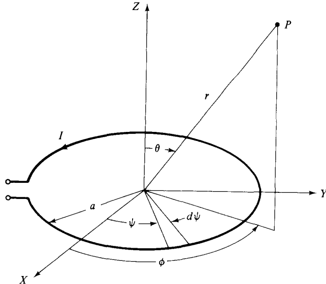
Fig. 2.8 The Small Current Loop
