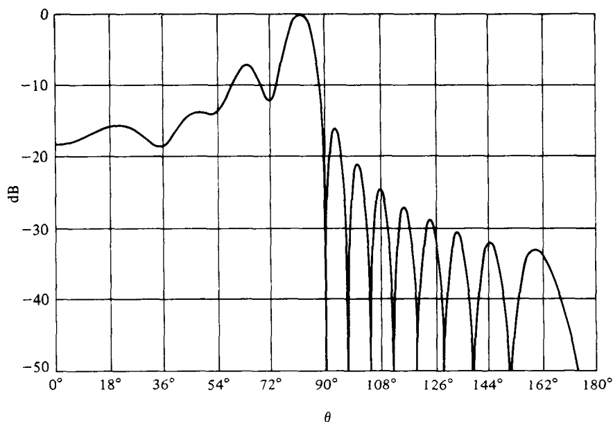
Fig. 5.29 Null-Filled Cosecant Squared Pattern
