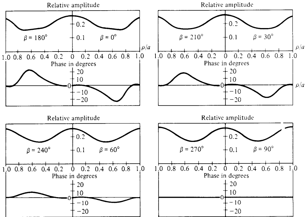
Fig. 6.13 The Continuous Aperture Distribution K(p, \beta) for the Sum Pattern of Fig. 6.12 (© 1975 IEEE. Reprinted from IEEE AP Transactions , pp. 523–527, 1975.)
