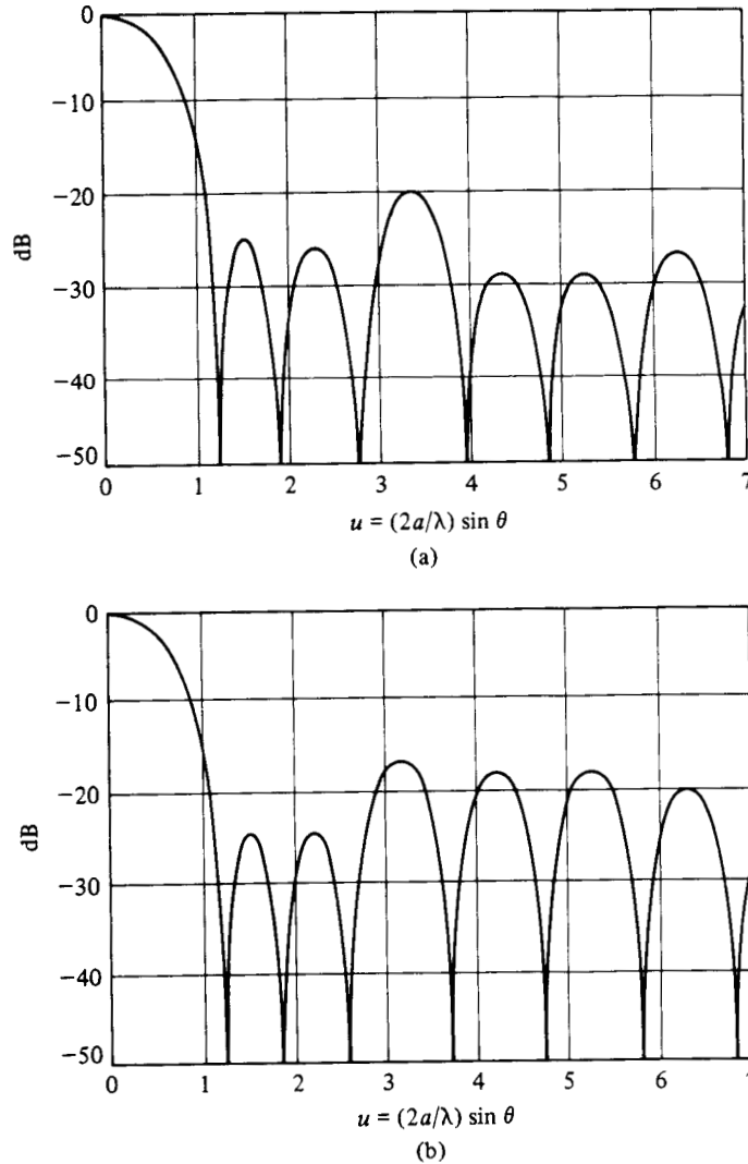
Fig. 6.22 The Sum Pattern for a Planar Array of Five Equispaced Concentric Continuous Ring Currents; a = 2.5\lambda ; Currents are Selected (a) to Match Pattern Nulls, and (b) After Perturbation to Match Side Lobe Heights of Fig. 6.10 (© 1978 Alta Frequenza. Reprinted from Graham, Johnson, and Elliott, Alta Frequenza , pp. 1-7, 1978.)
