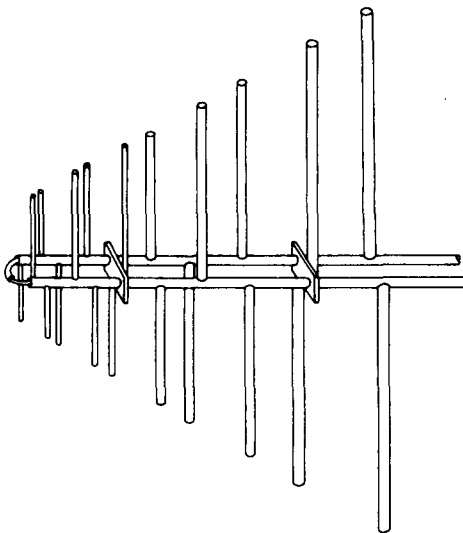
Fig. 8.27 A Properly Fed Log-Periodic Dipole Array
