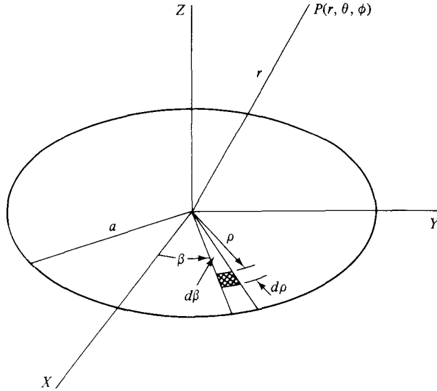
Fig. 6.6 Cartesian/Cylindrical/Spherical Coordinates
