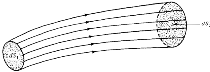
Fig. 10.2 A Tube of Geometrical Rays
