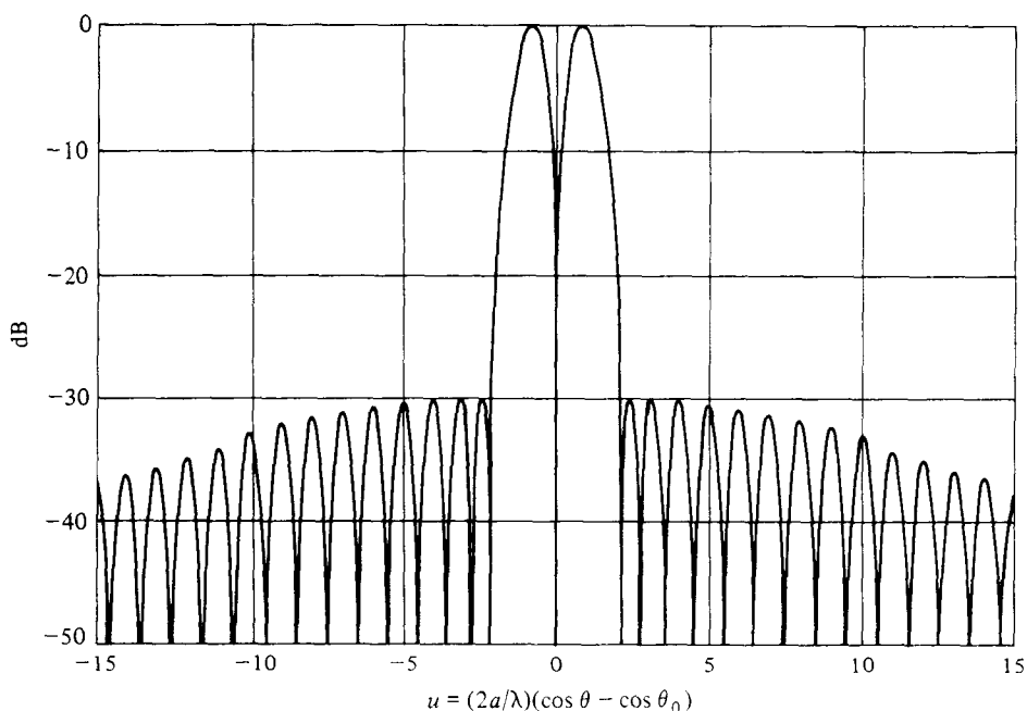
Fig. 5.22 Bayliss Difference Pattern for Continuous Line Source, n = 10 , -30 dB SLL (© 1976 IEEE. Reprinted from IEEE AP Transactions , pp. 310–316, 1976.)
