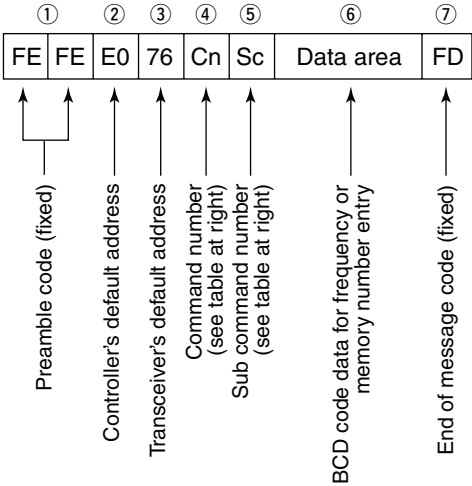
IC-7200 TO CONTROLLER
