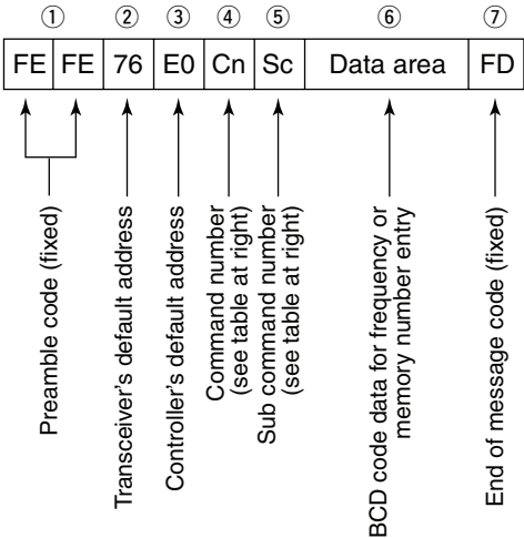
CONTROLLER TO IC-7200
