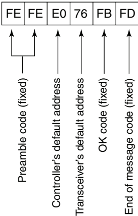
OK MESSAGE TO CONTROLLER
